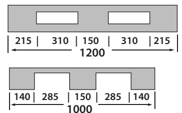
Forklift Entry Dimensions
